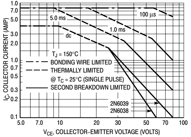
Figure 5. 2N6038, 2N6039
