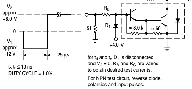
Figure 1. Switching Times Test Circuit
